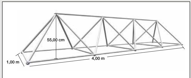
Trellis frame
